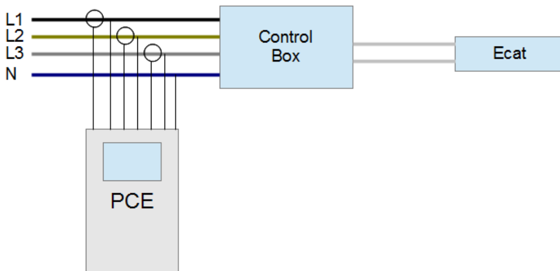
Fig. 1. Wiring diagram of the PCE-830 Power and Harmonics Analyzer. The three-phase power cables were checked and connected directly to the electrical outlet. It was established and verified that no other cable was present and that all connections were normal. The ground cable was disconnected before measurements began.
